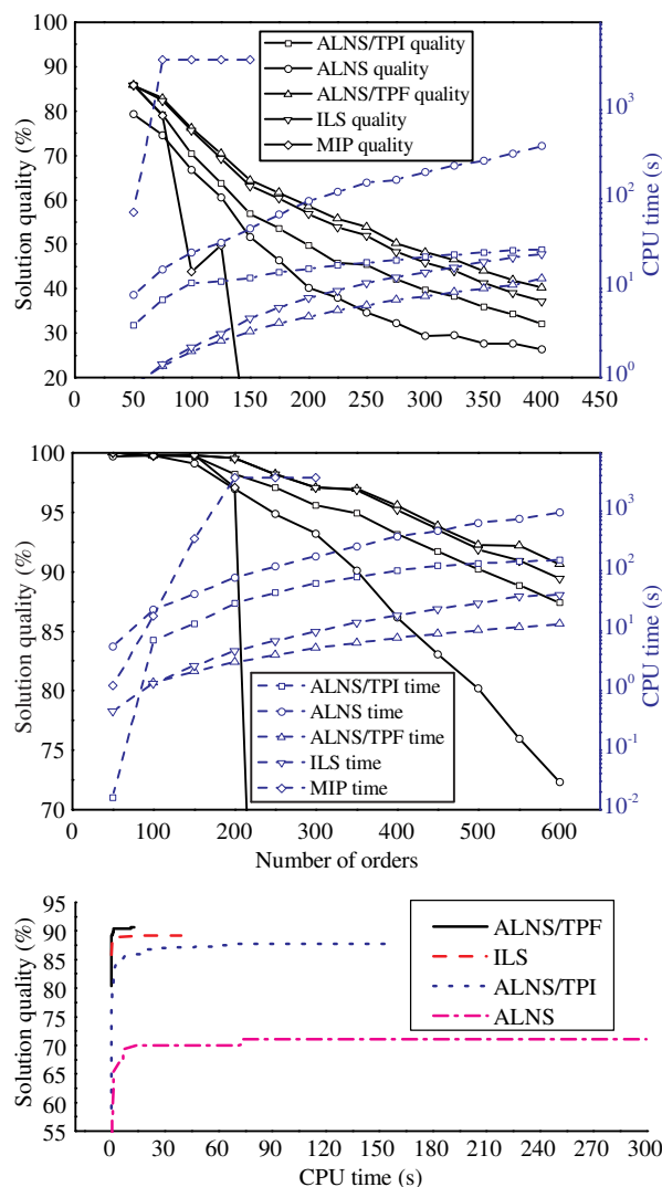
Figure 2: Comparison of algorithms on area distribution (top) and worldwide (middle) and the anytime quality of different algorithms (bottom) for the AEOSS problem
